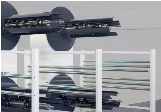
The guide rollers are adaptable in height, separating the sheet layers in order to protect the material surfaces.
